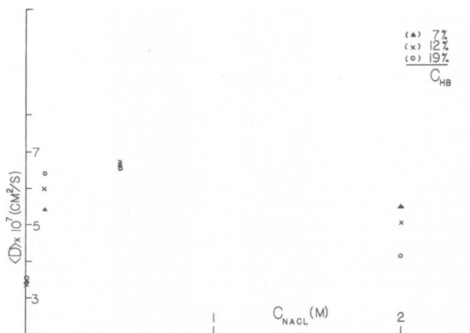
FIGURE 11 \langle D \rangle vs. CNaCl for oxy-HbA, pH = 6.7, at various values of CHb.
